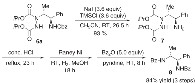
Scheme 1. Synthesis of trans -1,2-diamine derivatives 7 and 8 . Cbz = carbobenzyloxy, TMS = trimethylsilyl, Bz = benzoyl.
